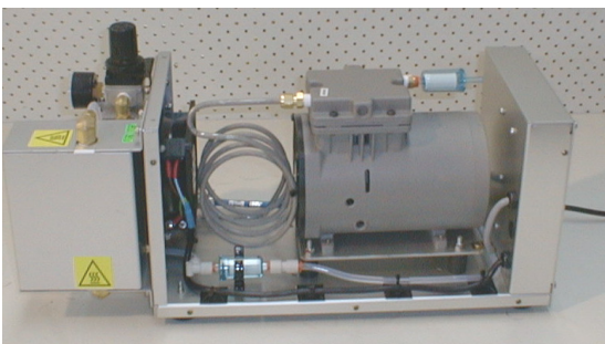
8301LC Zero Air Generator
